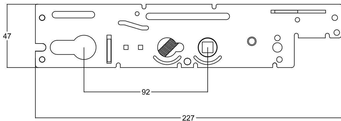
FULLEX-XL-35-SLAVE-CASE 35mm backset centre case inline slave door
